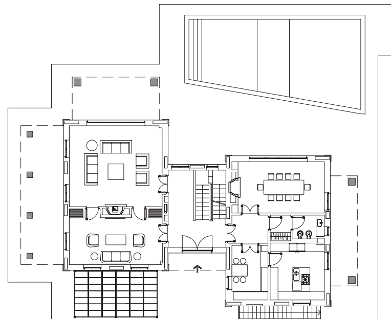
Piano terra
